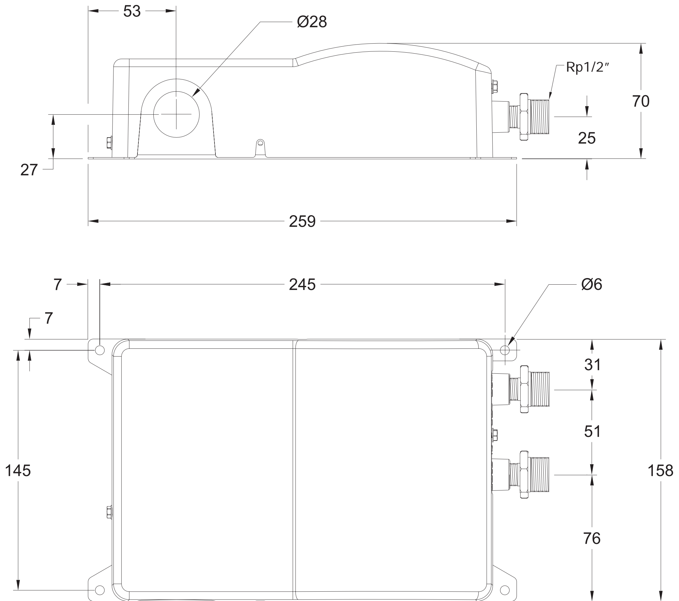
Chronomite Dimensions
